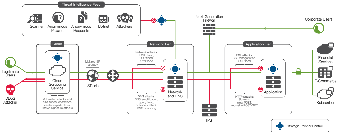
Figure 2: F5 recommends a multi-tiered DDoS approach to your architecture.
